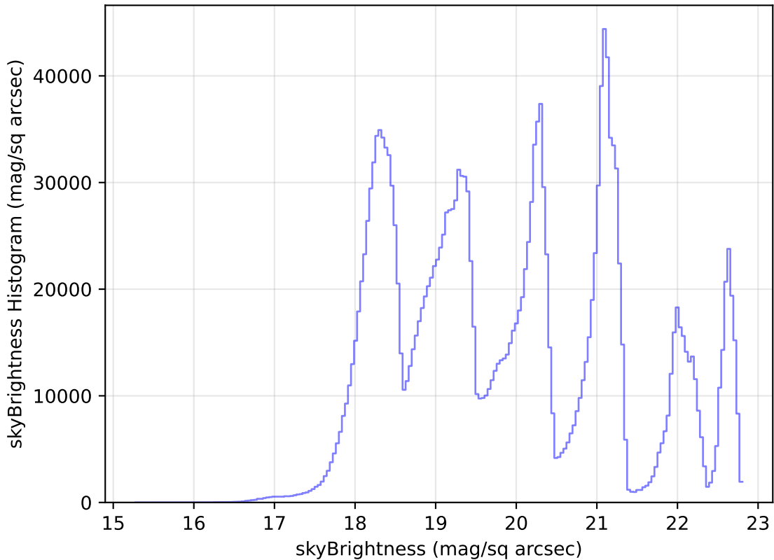
weather_cloudso10v3.4_10yrs All sky all bands: skyBrightness Histogram
