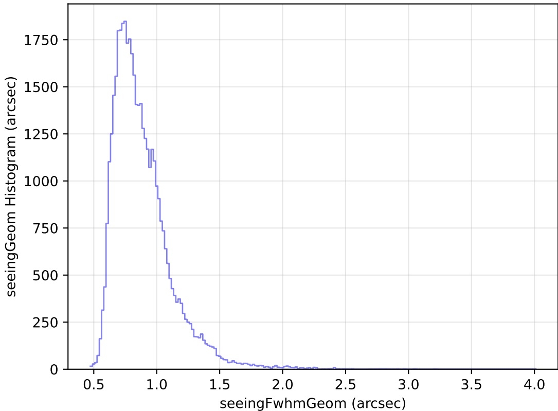
weather_cloudso10v3.4_10yrs Yr 1 z band: seeingGeom Histogram
