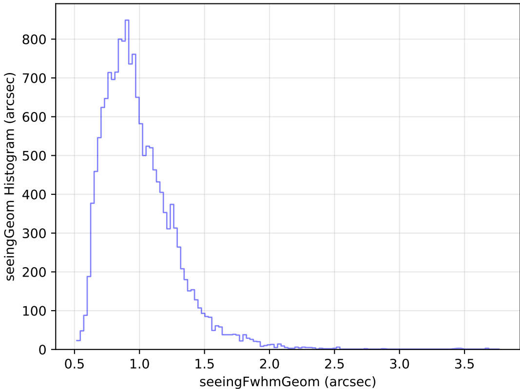
weather_cloudso10v3.4_10yrs Yr 1 u band: seeingGeom Histogram
