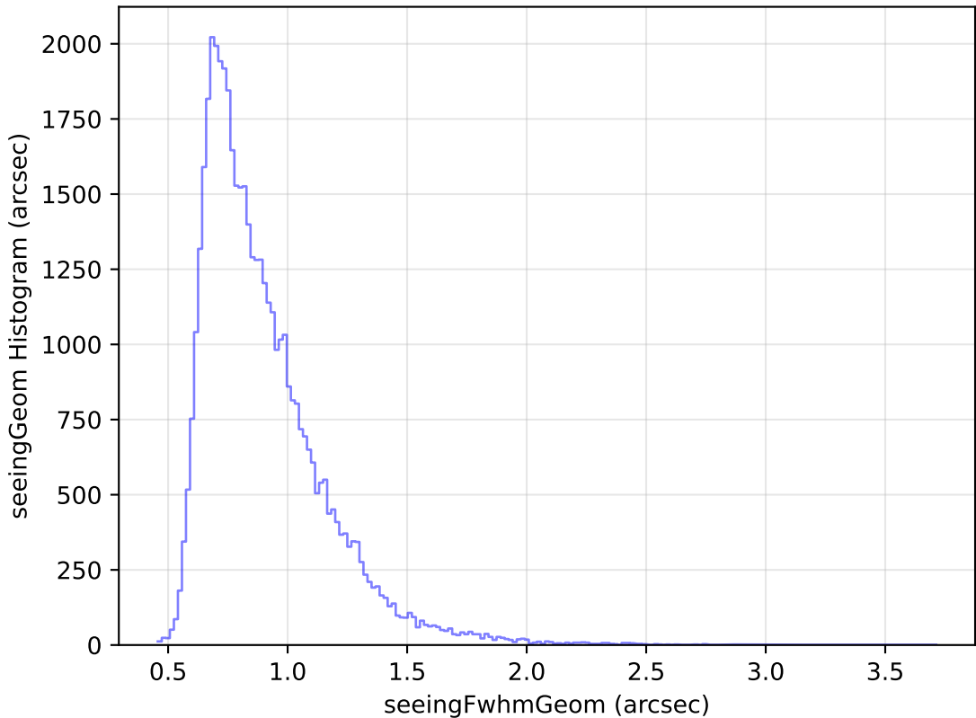
weather_cloudso10v3.4_10yrs Yr 1 r band: seeingGeom Histogram
