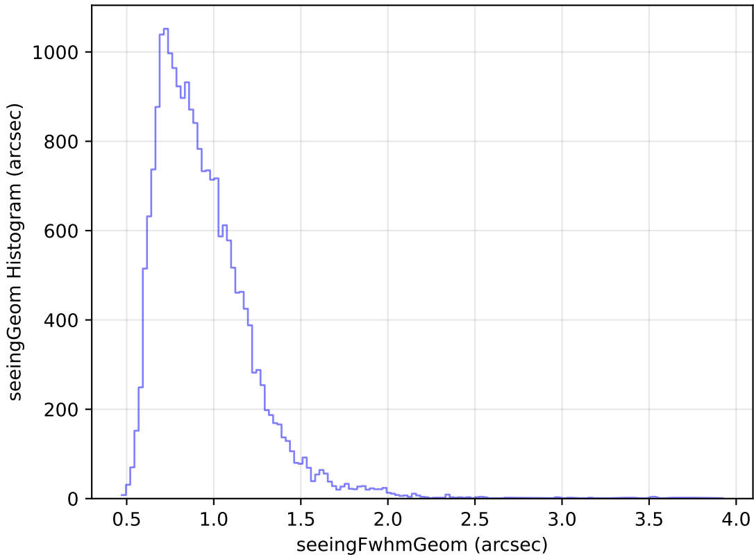
weather_cloudso10v3.4_10yrs Yr 1 g band: seeingGeom Histogram
