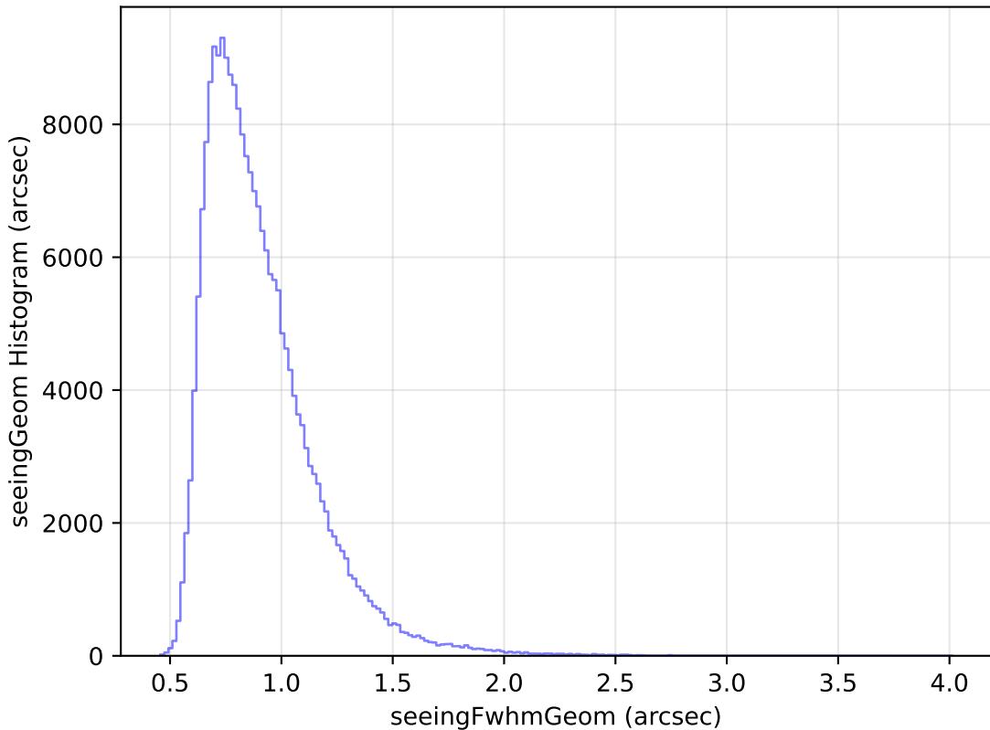
weather_cloudso10v3.4_10yrs Yr 1 all bands: seeingGeom Histogram
