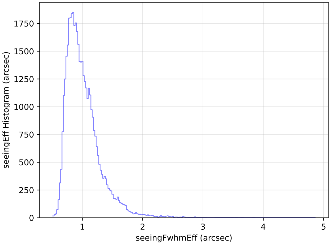
weather_cloudso10v3.4_10yrs Yr 1 z band: seeingEff Histogram
