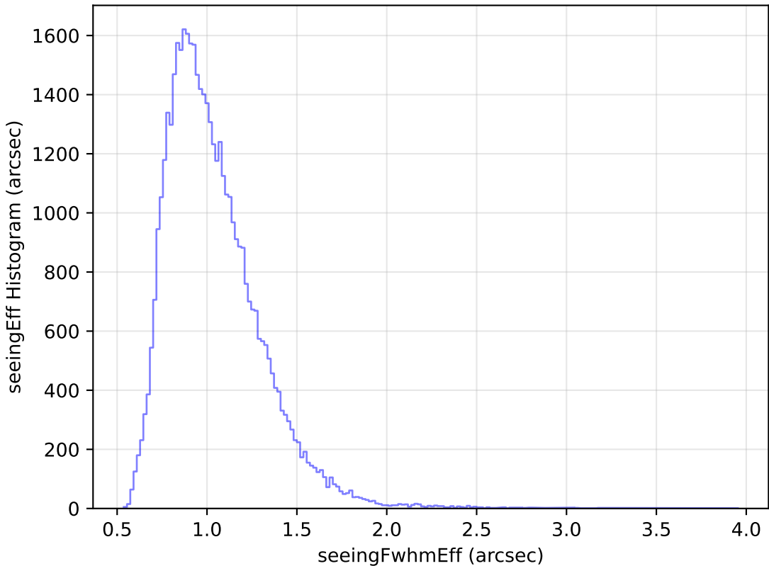
weather_cloudso10v3.4_10yrs Yr 1 y band: seeingEff Histogram
