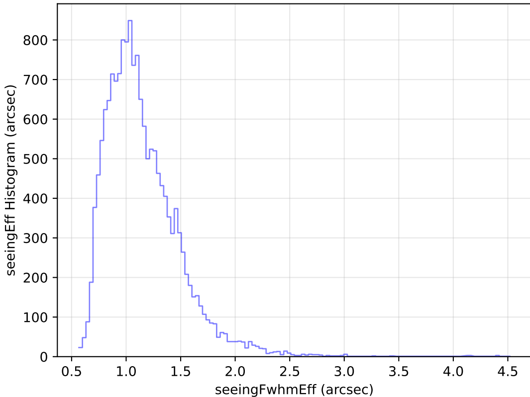
weather_cloudso10v3.4_10yrs Yr 1 u band: seeingEff Histogram
