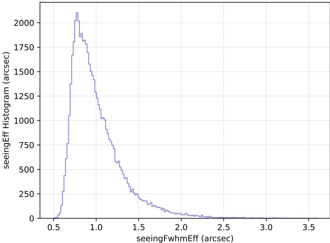
weather_cloudso10v3.4_10yrs Yr 1 i band: seeingEff Histogram
