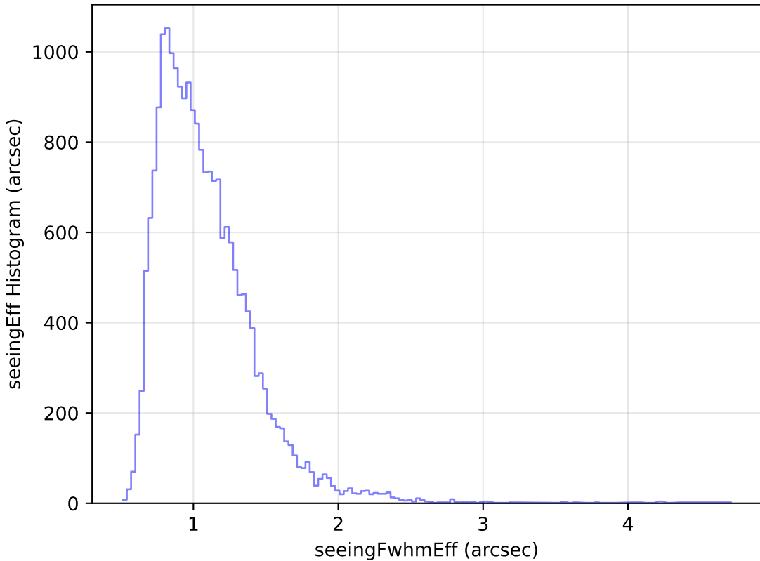
weather_cloudso10v3.4_10yrs Yr 1 g band: seeingEff Histogram
