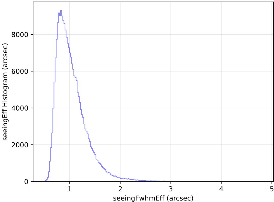
weather_cloudso10v3.4_10yrs Yr 1 all bands: seeingEff Histogram
