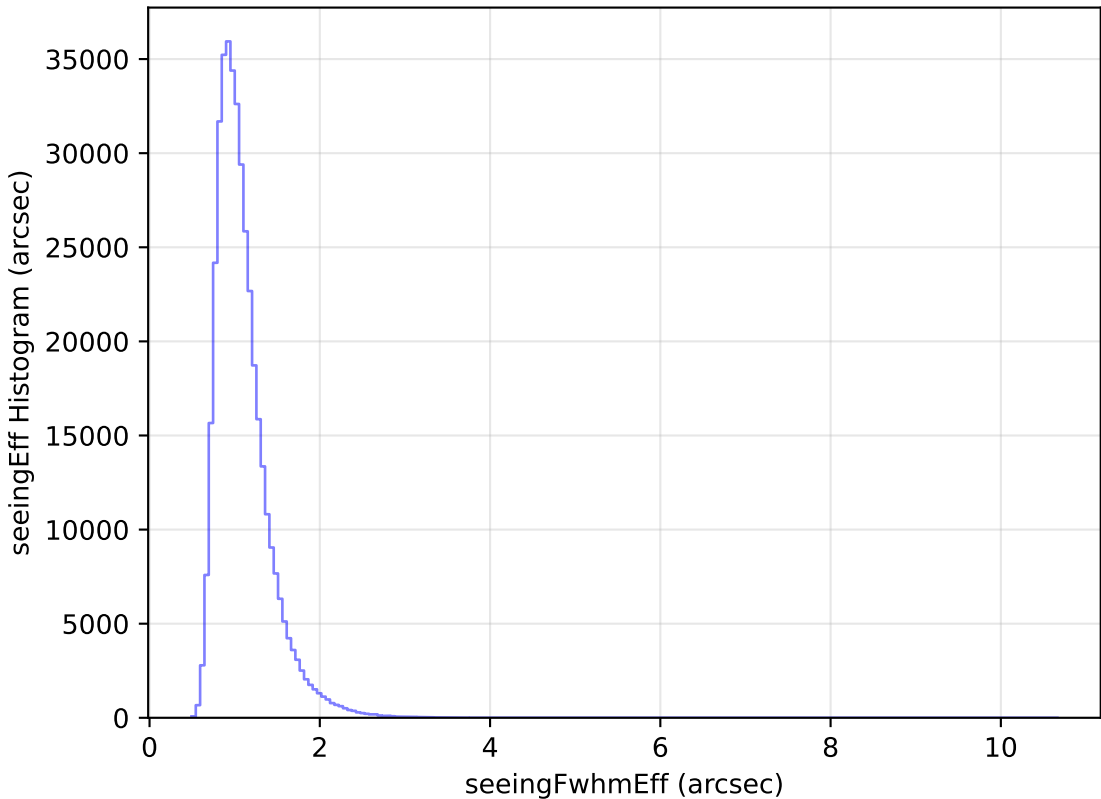
weather_cloudso10v3.4_10yrs WFD y band: seeingEff Histogram
