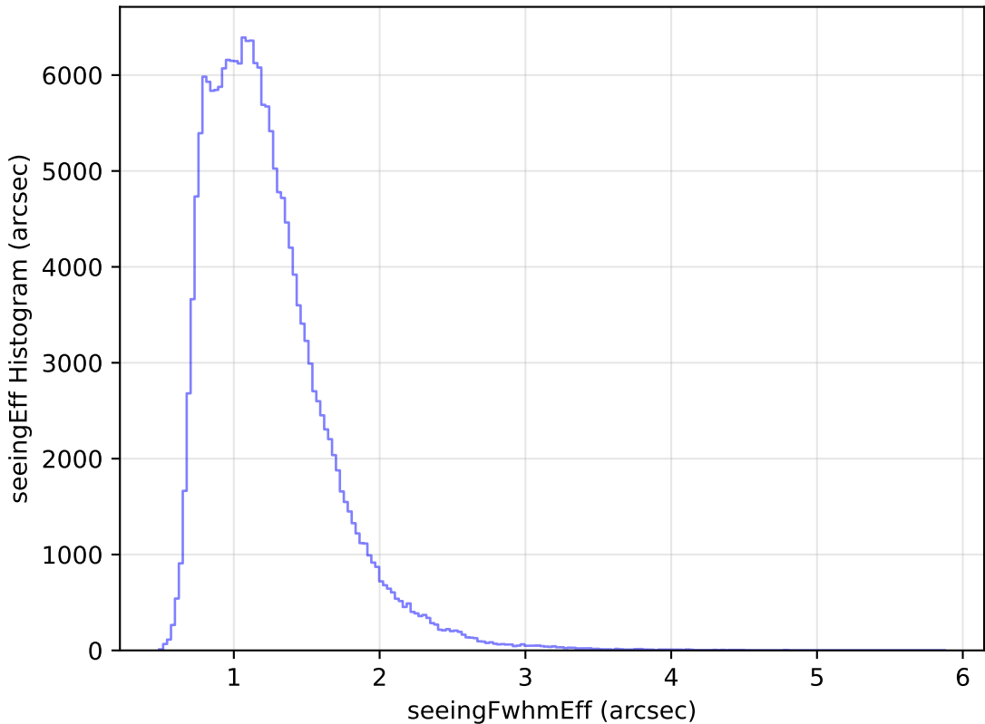
weather_cloudso10v3.4_10yrs WFD g band: seeingEff Histogram
