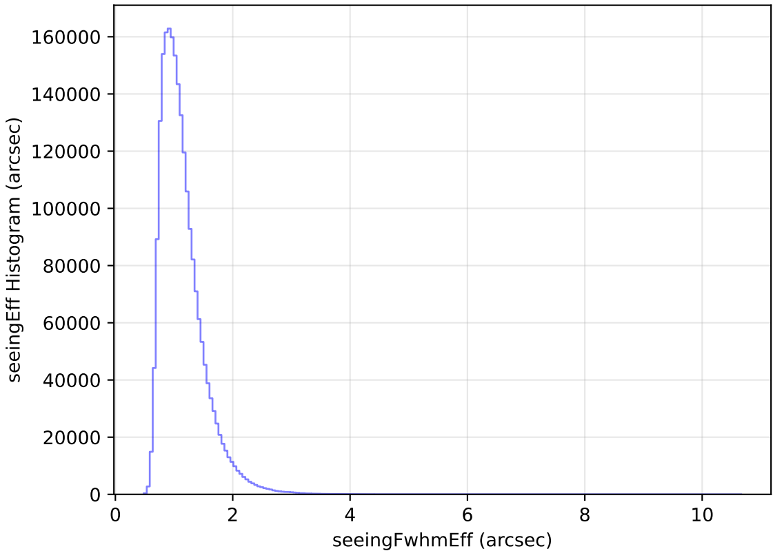
weather_cloudso10v3.4_10yrs WFD all bands: seeingEff Histogram
