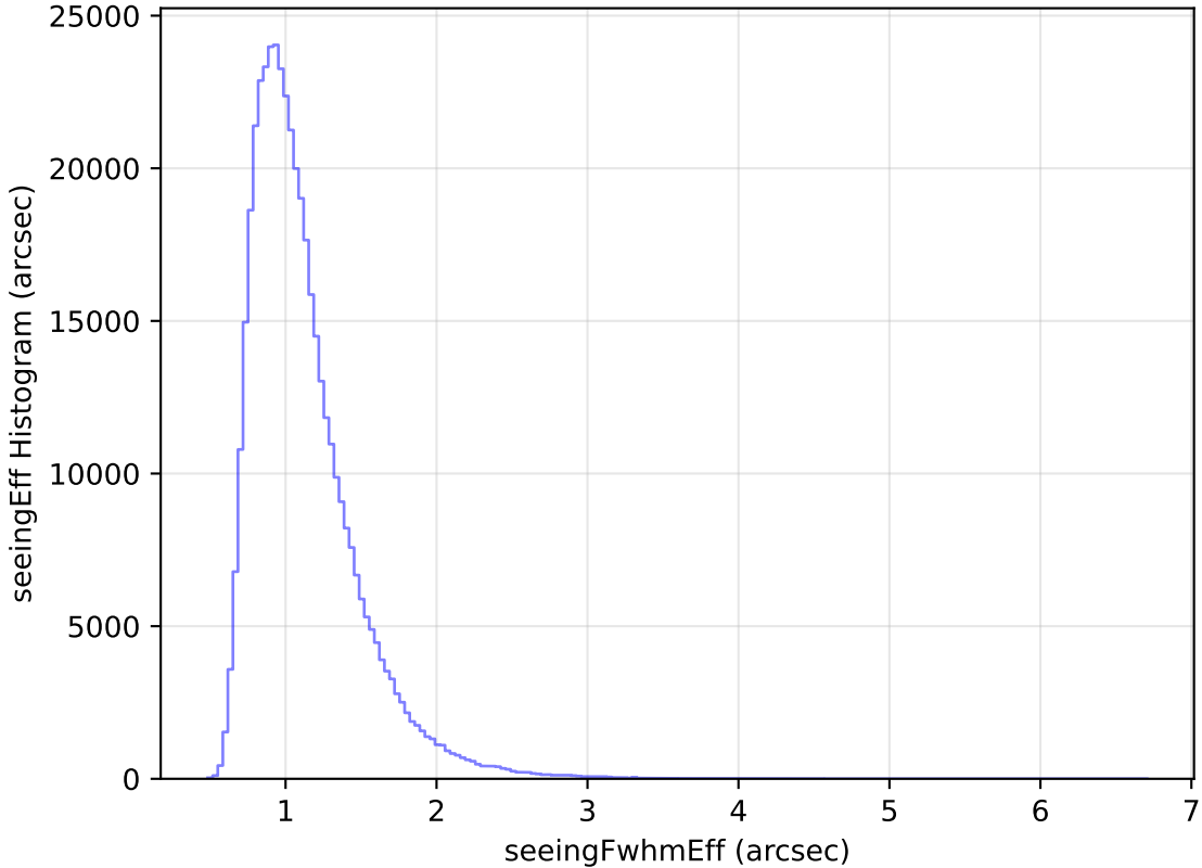
weather_cloudso10v3.4_10yrs All sky z band: seeingEff Histogram
