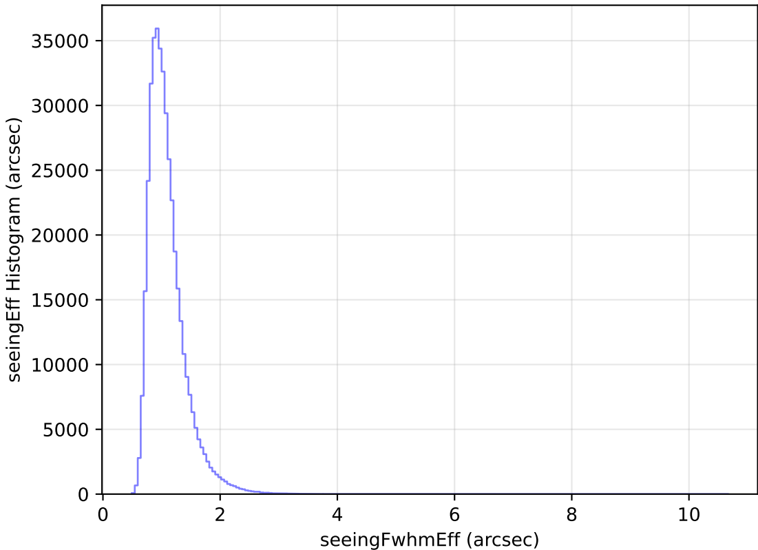
weather_cloudso10v3.4_10yrs All sky y band: seeingEff Histogram
