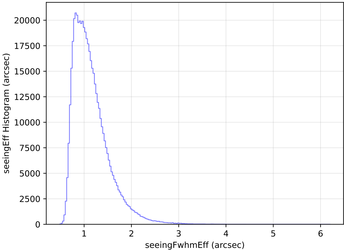
weather_cloudso10v3.4_10yrs All sky r band: seeingEff Histogram
