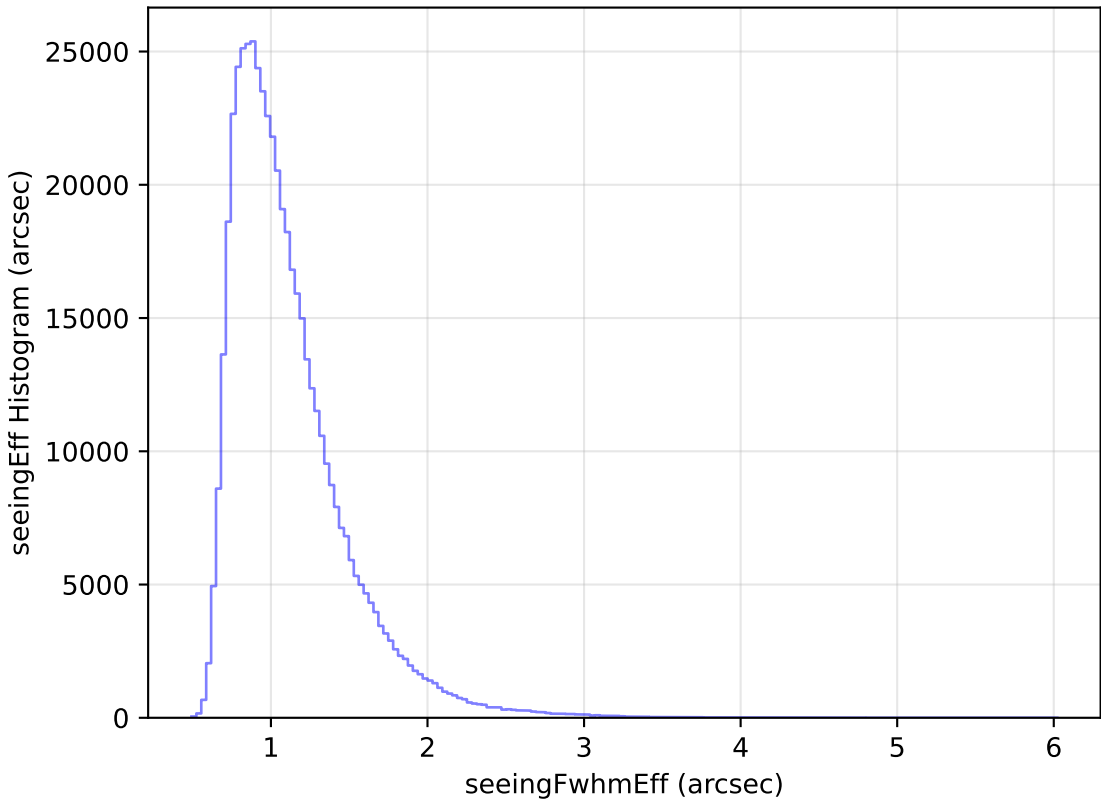
weather_cloudso10v3.4_10yrs All sky i band: seeingEff Histogram
