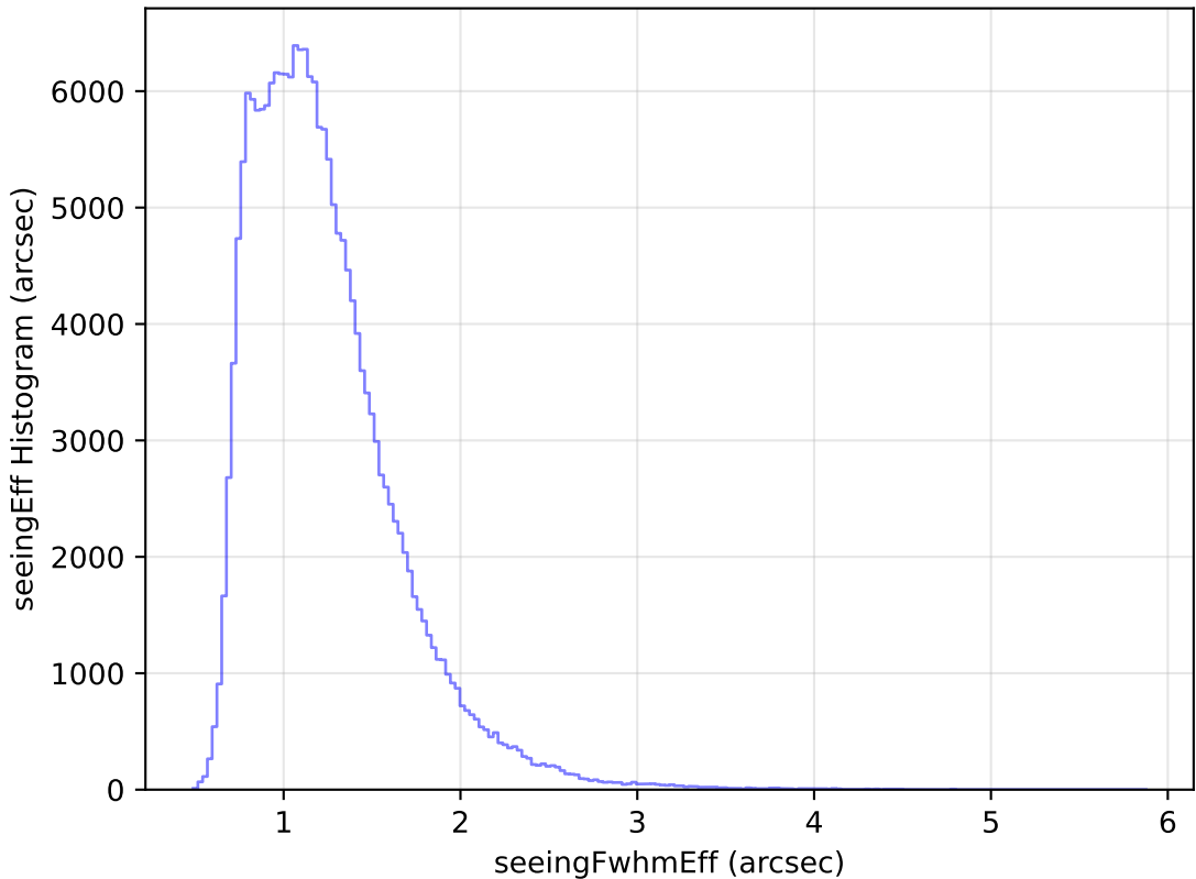
weather_cloudso10v3.4_10yrs All sky g band: seeingEff Histogram
