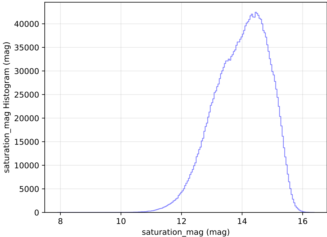
weather_cloudso10v3.4_10yrs WFD all bands: saturation_mag Histogram
