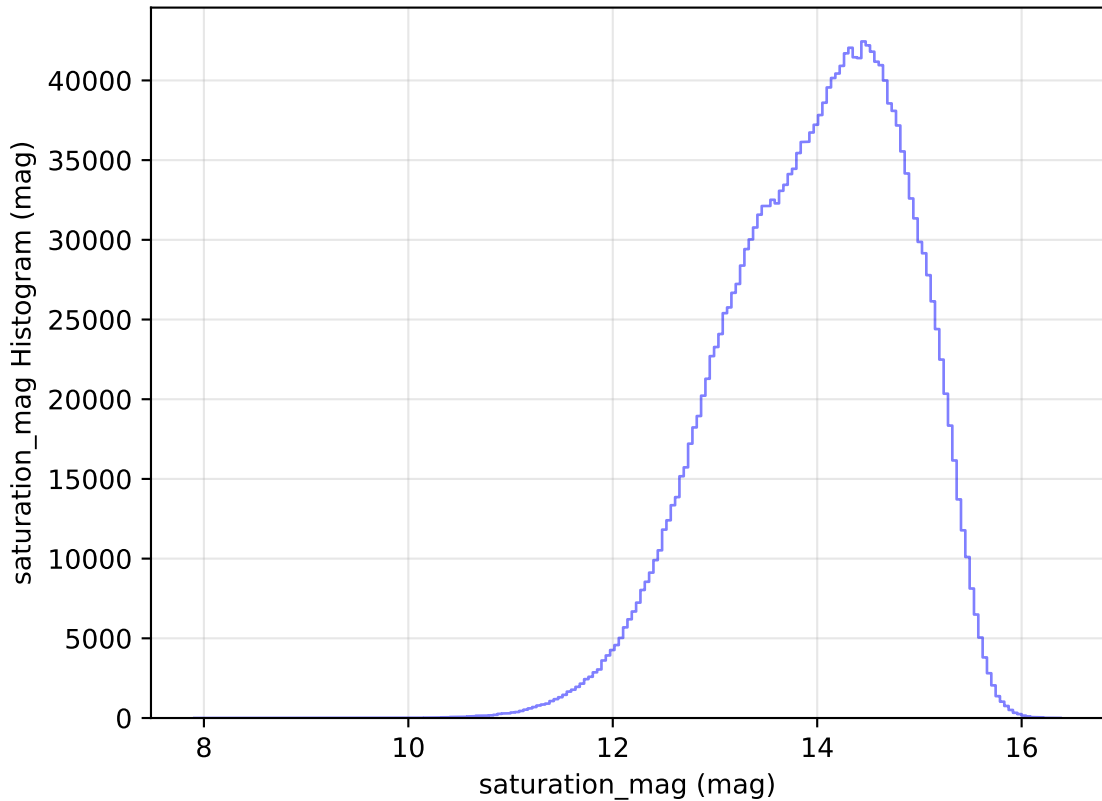
weather_cloudso10v3.4_10yrs All sky all bands: saturation_mag Histogram
