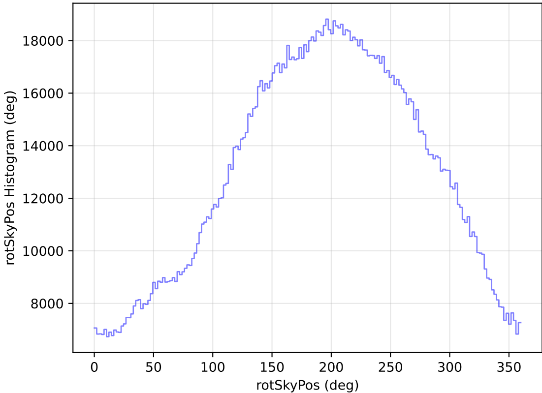
weather_cloudso10v3.4_10yrs WFD all bands: rotSkyPos Histogram
