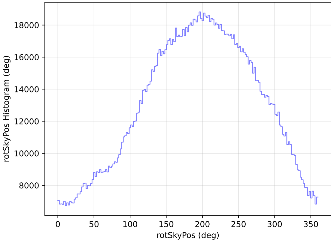
weather_cloudso10v3.4_10yrs All sky all bands: rotSkyPos Histogram
