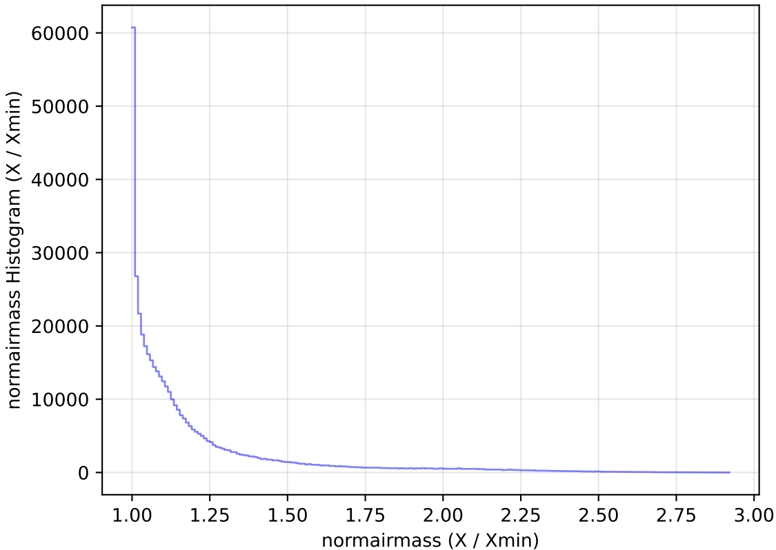
weather_cloudso10v3.4_10yrs WFD z band: normairmass Histogram
