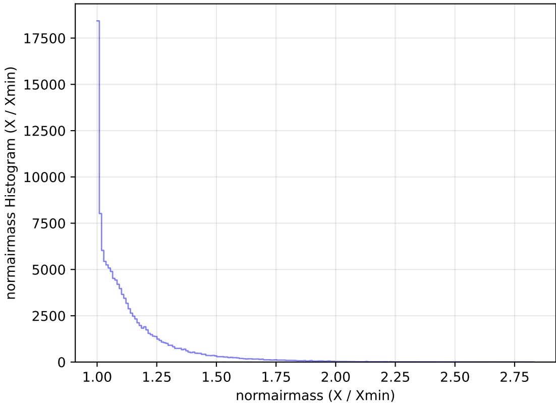
weather_cloudso10v3.4_10yrs WFD u band: normairmass Histogram
