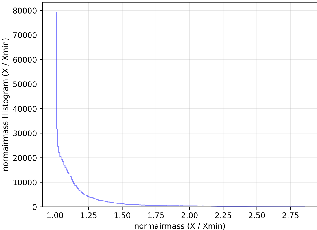
weather_cloudso10v3.4_10yrs WFD r band: normairmass Histogram
