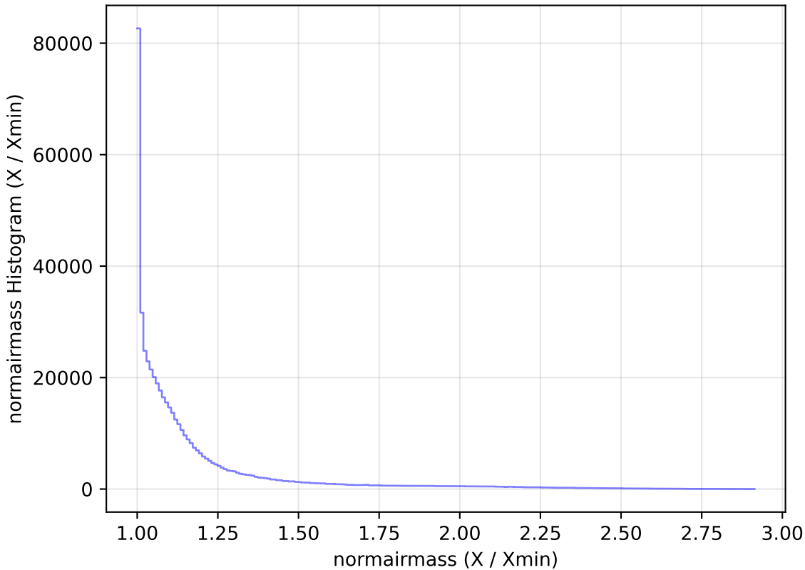
weather_cloudso10v3.4_10yrs WFD i band: normairmass Histogram
