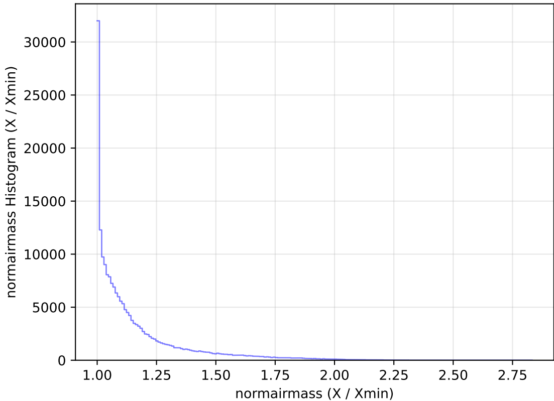
weather_cloudso10v3.4_10yrs WFD g band: normairmass Histogram
