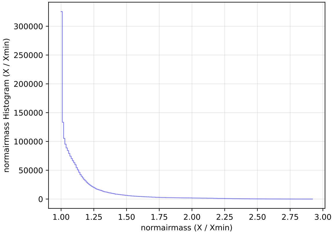
weather_cloudso10v3.4_10yrs WFD all bands: normairmass Histogram
