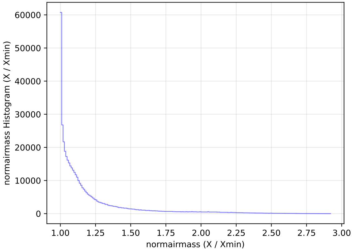
weather_cloudso10v3.4_10yrs All sky z band: normairmass Histogram
