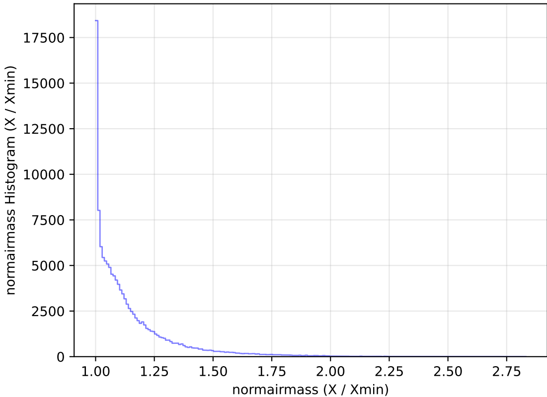
weather_cloudso10v3.4_10yrs All sky u band: normairmass Histogram
