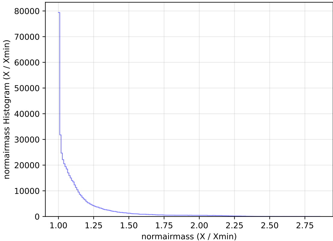
weather_cloudso10v3.4_10yrs All sky r band: normairmass Histogram
