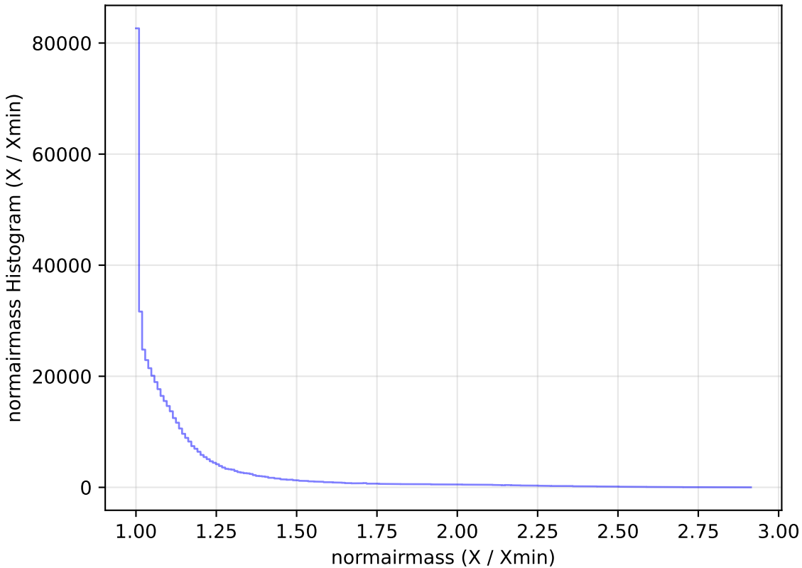
weather_cloudso10v3.4_10yrs All sky i band: normairmass Histogram
