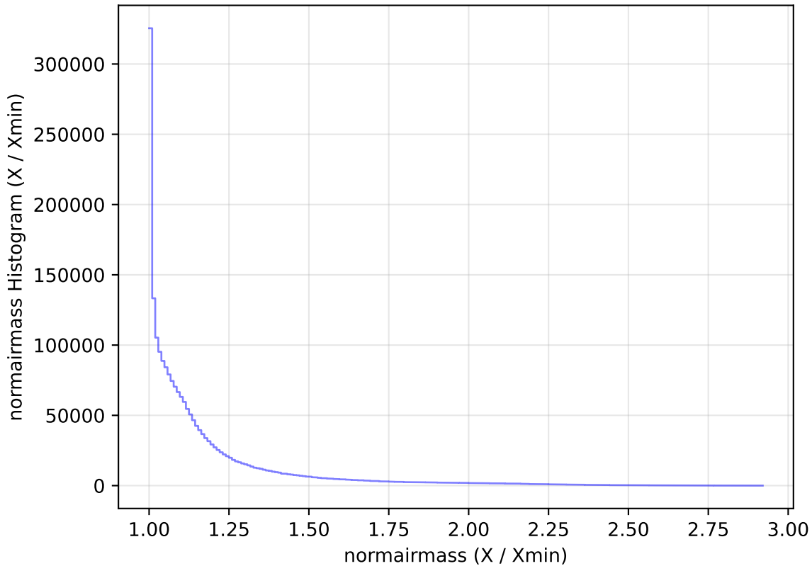
weather_cloudso10v3.4_10yrs All sky all bands: normairmass Histogram
