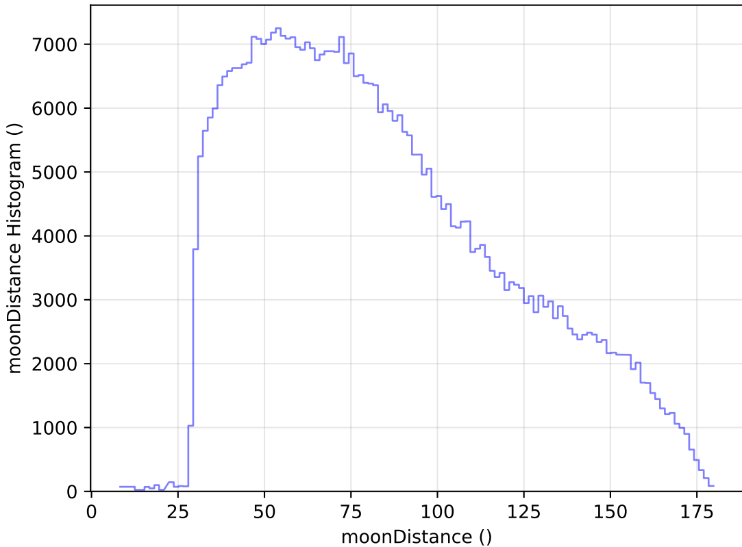
weather_cloudso10v3.4_10yrs WFD z band: moonDistance Histogram
