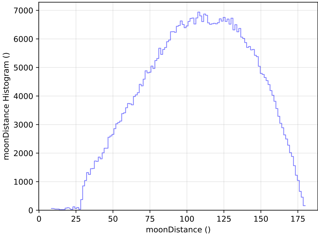
weather_cloudso10v3.4_10yrs WFD r band: moonDistance Histogram
