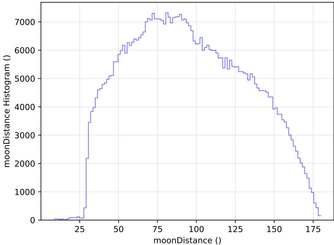
weather_cloudso10v3.4_10yrs WFD i band: moonDistance Histogram
