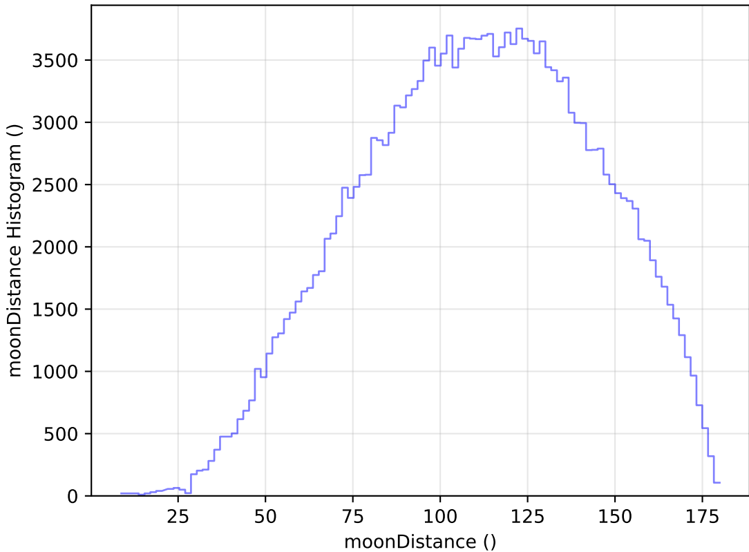
weather_cloudso10v3.4_10yrs WFD g band: moonDistance Histogram
