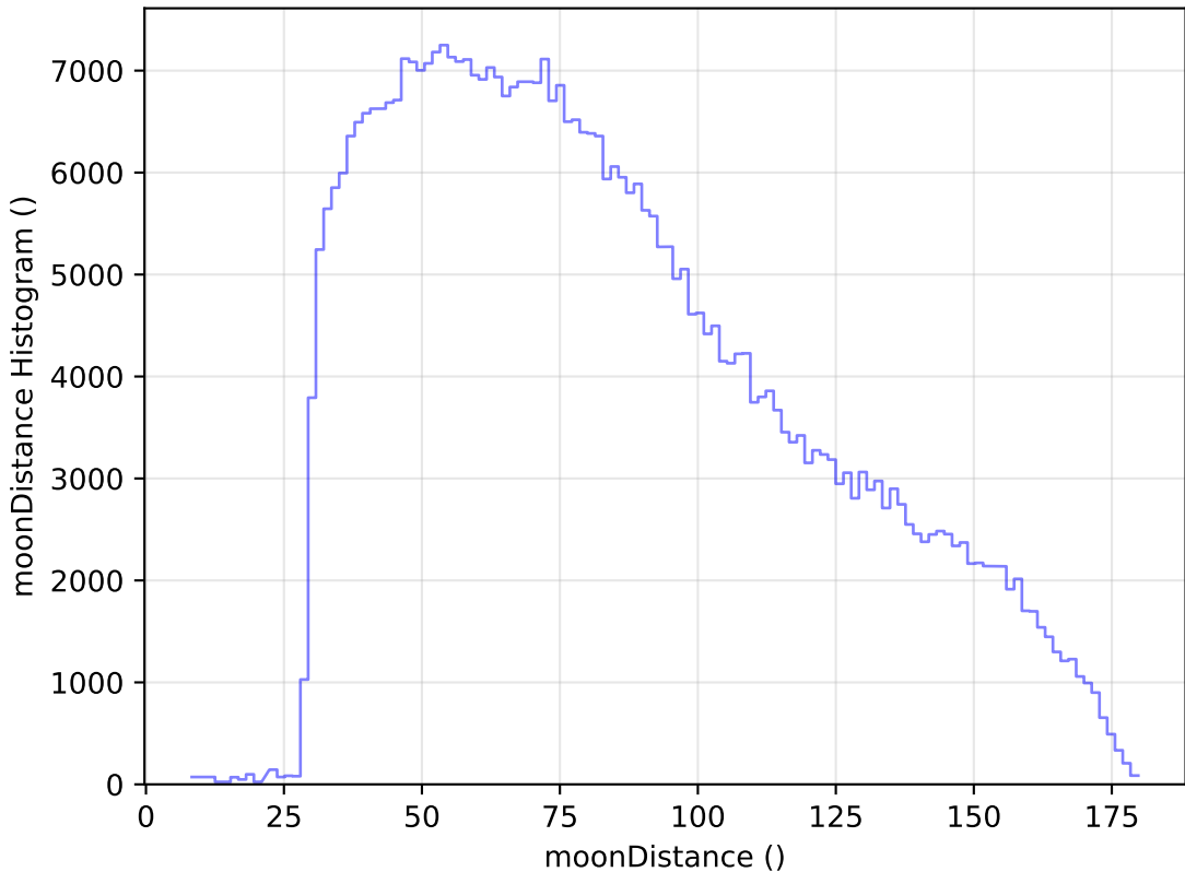
weather_cloudso10v3.4_10yrs All sky z band: moonDistance Histogram
