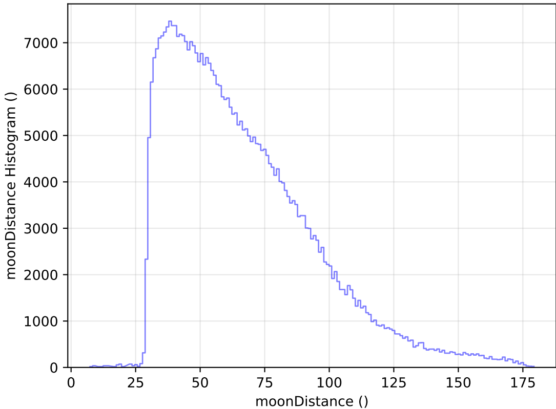
weather_cloudso10v3.4_10yrs All sky y band: moonDistance Histogram
