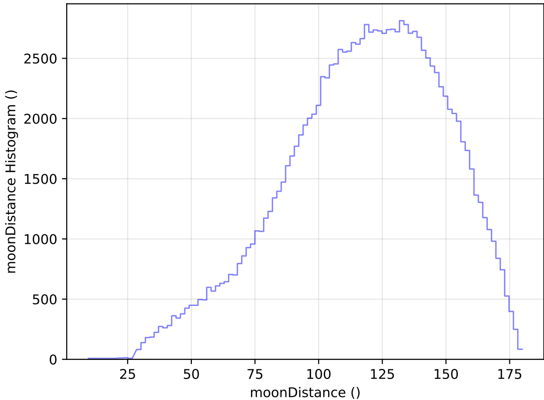
weather_cloudso10v3.4_10yrs All sky u band: moonDistance Histogram
