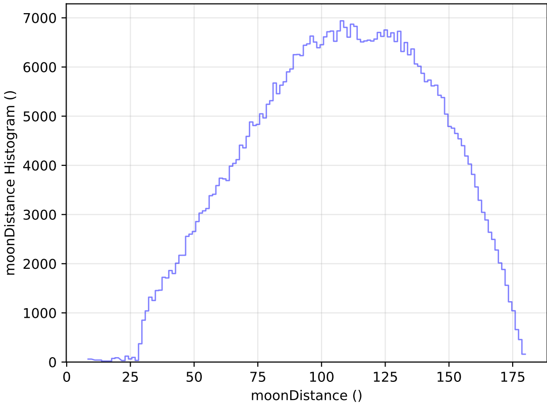
weather_cloudso10v3.4_10yrs All sky r band: moonDistance Histogram
