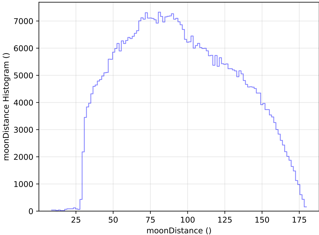
weather_cloudso10v3.4_10yrs All sky i band: moonDistance Histogram
