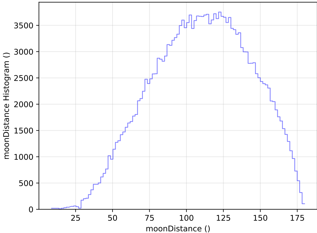
weather_cloudso10v3.4_10yrs All sky g band: moonDistance Histogram
