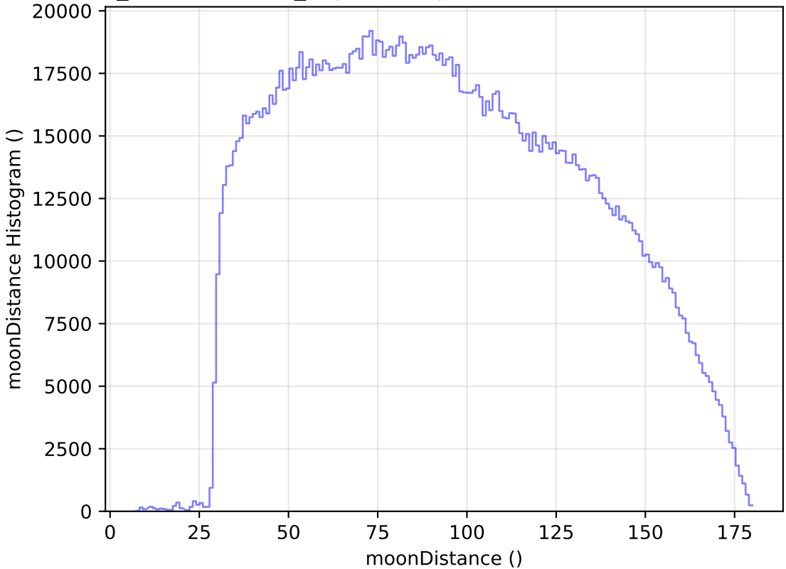
weather_cloudso10v3.4_10yrs All sky all bands: moonDistance Histogram
