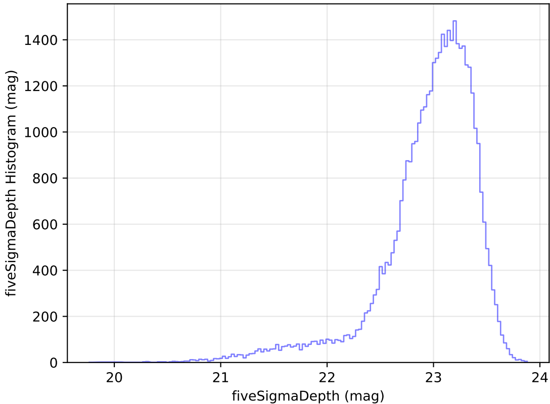
weather_cloudso10v3.4_10yrs Yr 1 z band: fiveSigmaDepth Histogram
