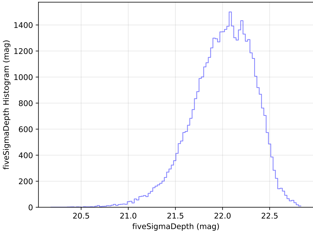
weather_cloudso10v3.4_10yrs Yr 1 y band: fiveSigmaDepth Histogram
