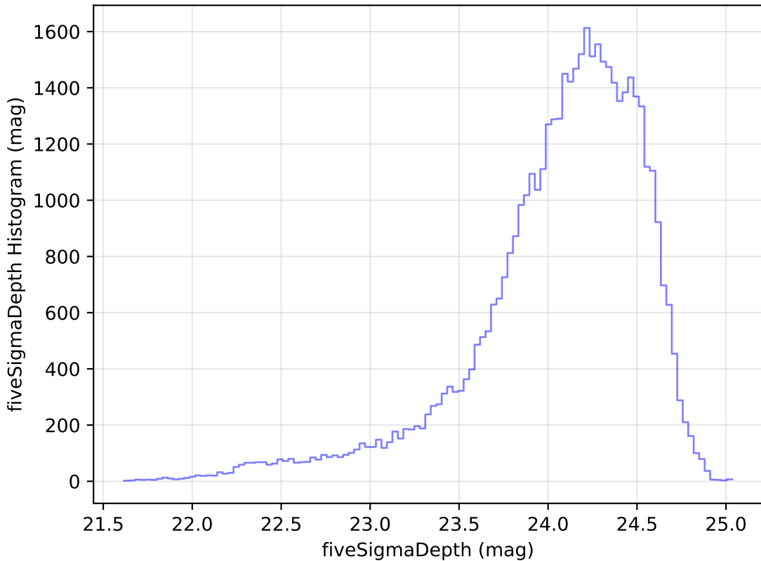
weather_cloudso10v3.4_10yrs Yr 1 r band: fiveSigmaDepth Histogram
