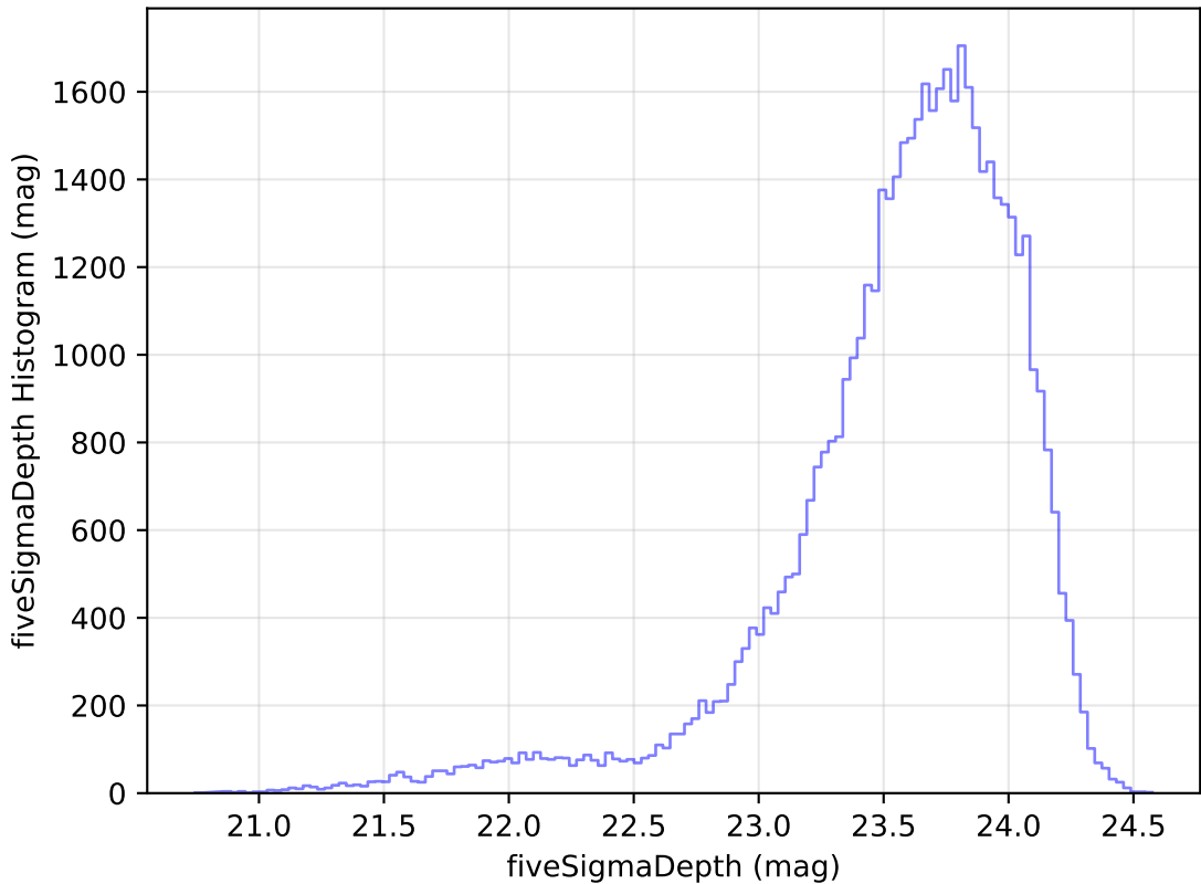
weather_cloudso10v3.4_10yrs Yr 1 i band: fiveSigmaDepth Histogram
